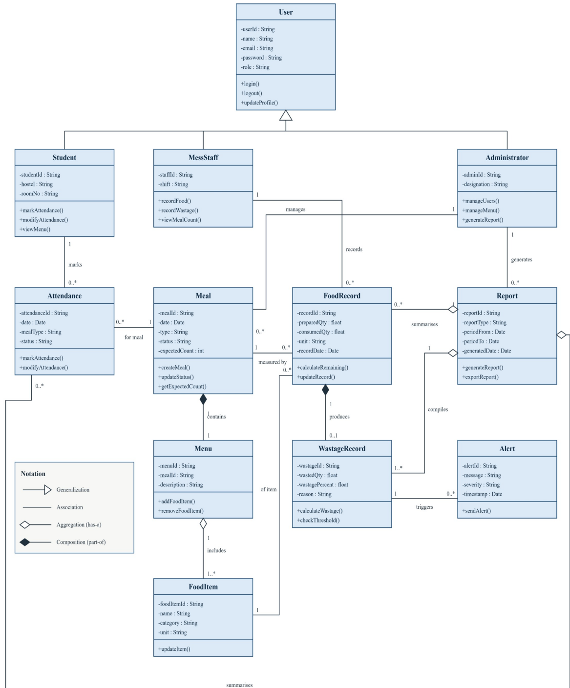
Figure 8.6: Class Diagram
